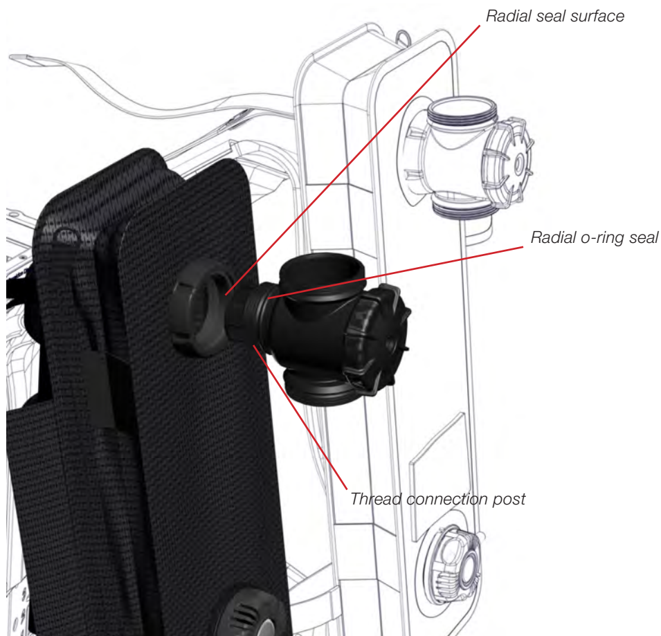
Figure A2-4. Insert the right hand water diversion manifold into the port on the right counterlung. Clockwise tighten the water diversion manifold into the right and left counterlung shoulder port. Note the correct orientation, further described in chapter 1, section 4.
